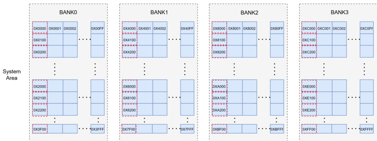
Fig .2 DRAM address map
